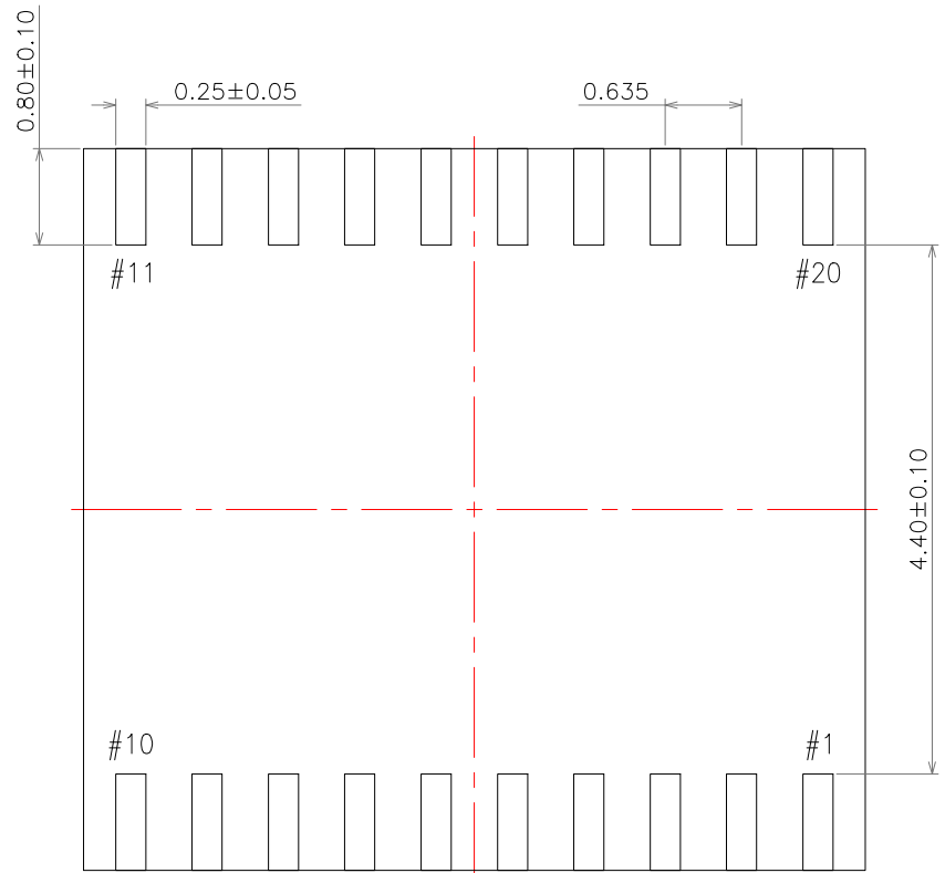
BOTTOM VIEW
